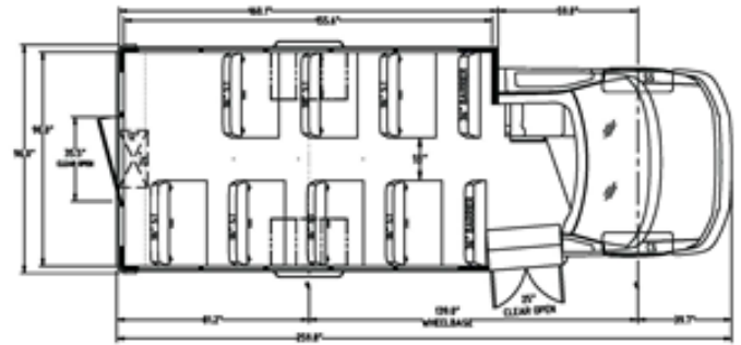
14 PASS + DRIVER SCHOOL BUS SEATS
