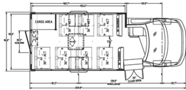
14 PASS + DRIVER ACTIVITY SEATS & CARGO
